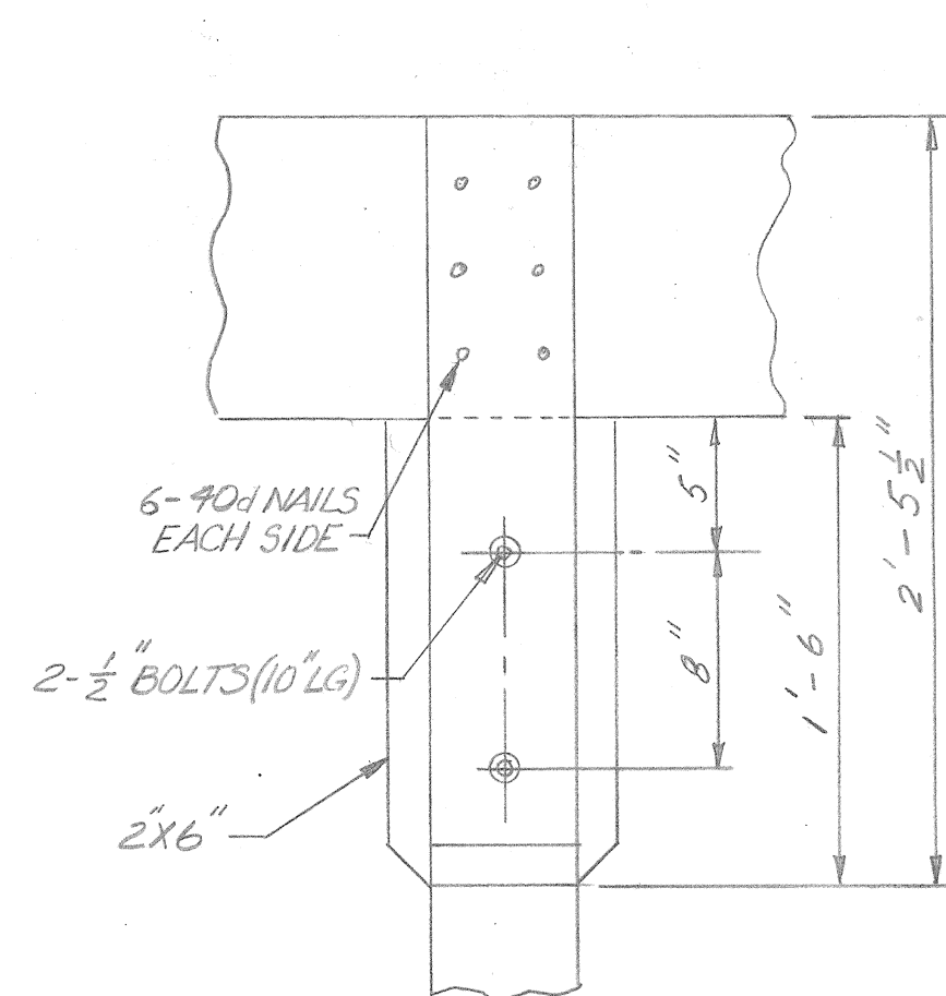
POST & GIRDER DETAIL
