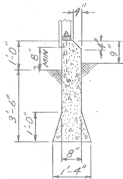
DETAIL AT ANCHOR BOLT
