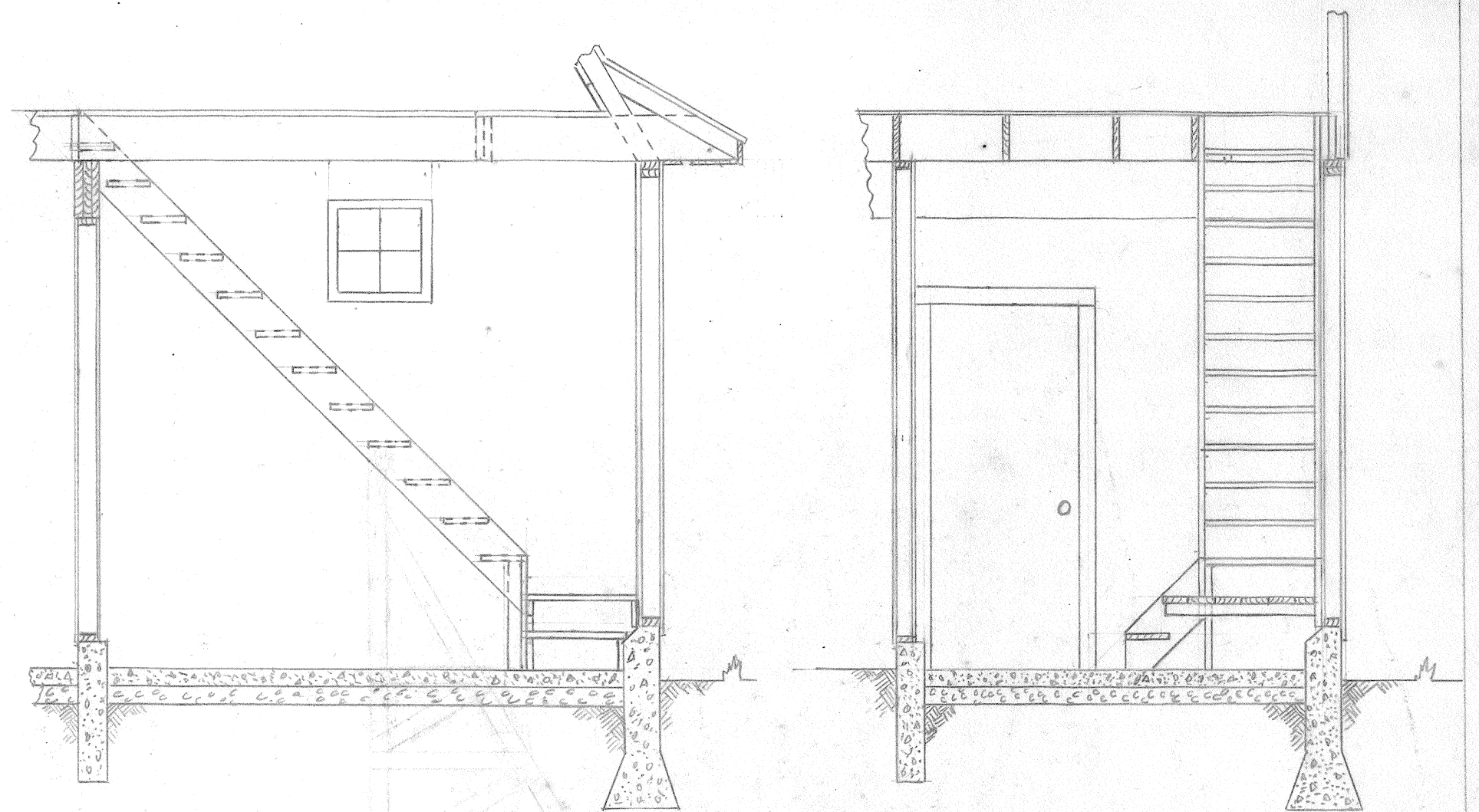
STAIRWAY ELEVATION
