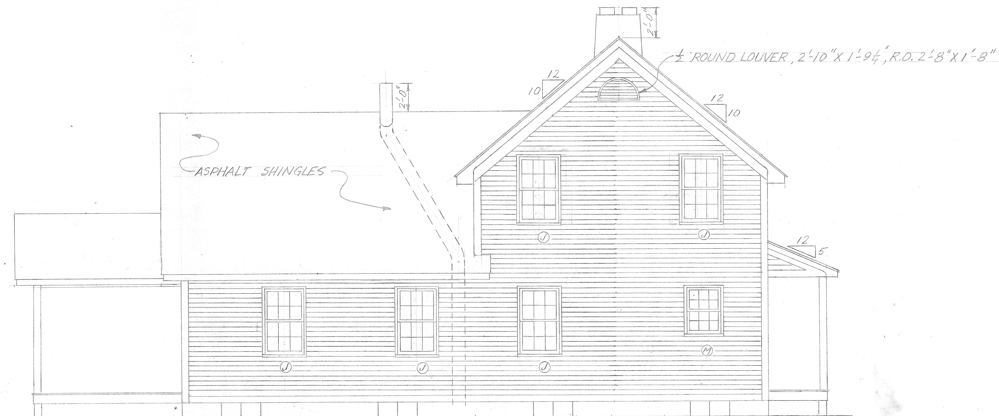
EAST ELEVATION 1/4" = 1'-0"
