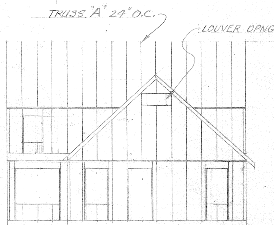
SOUTH ELEVATION FRAMING PLAN 1/8" = 1'-0"
