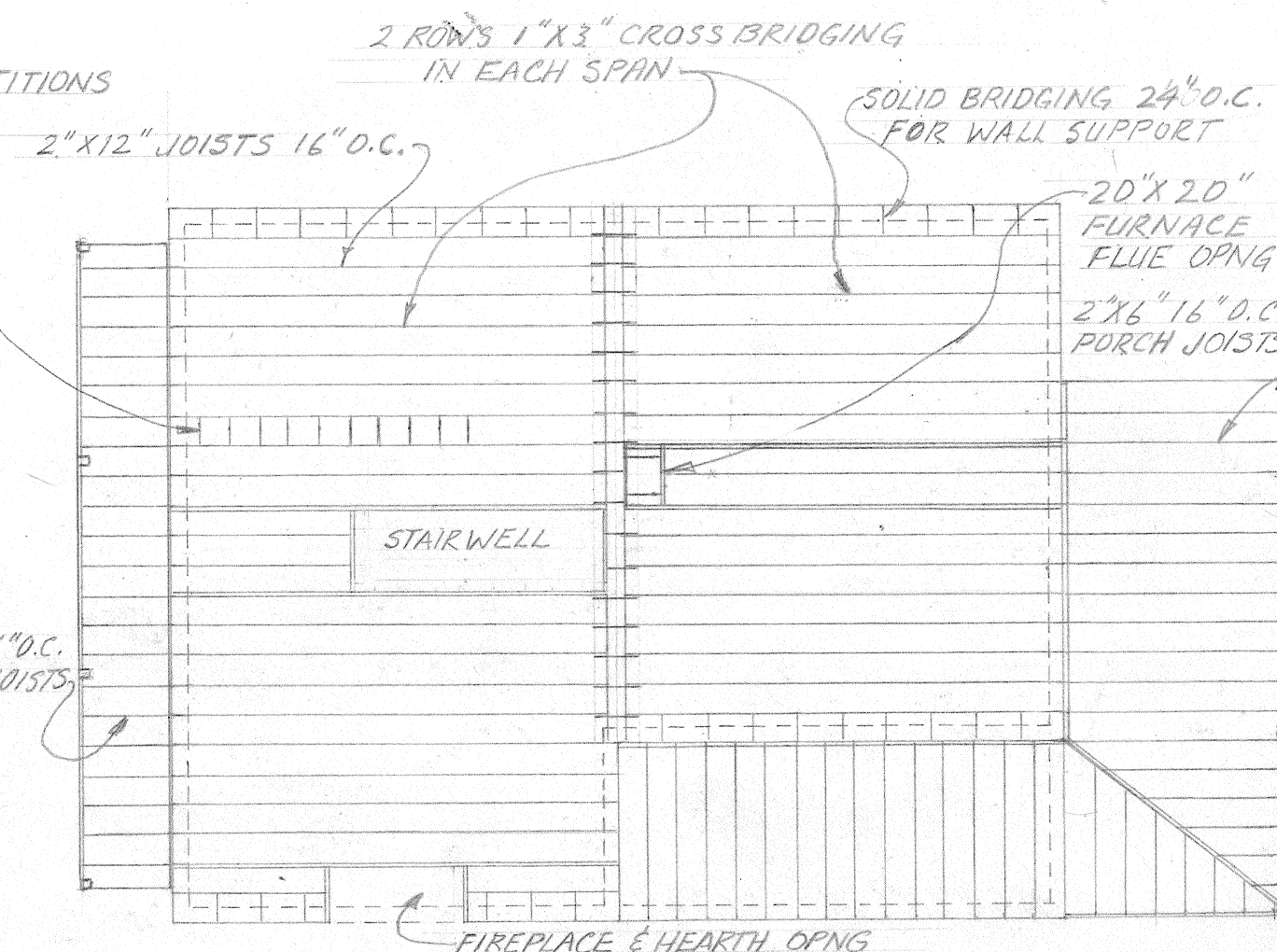
FIRST FLOOR JOISTS FRAMING PLAN 1/8" = 1'-0"
