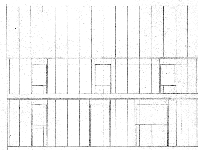
NORTH ELEVATION FRAMING PLAN 1/8" = 1'-0"
